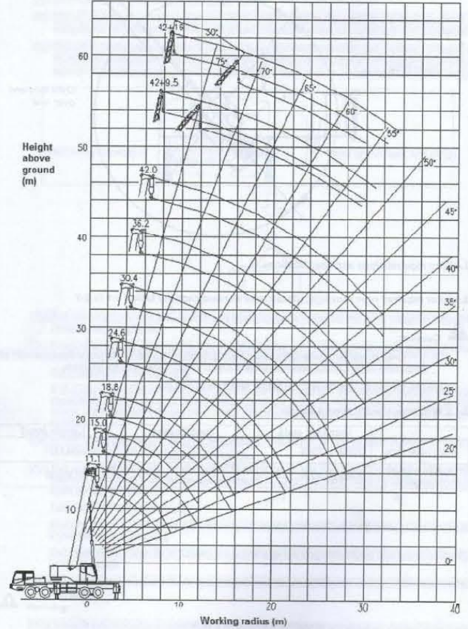
Lifting height curve
